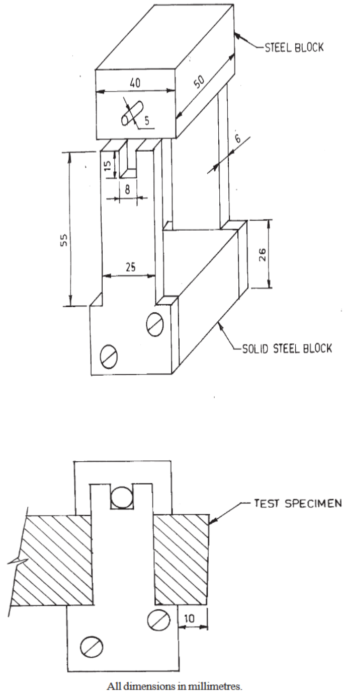
Figure 2-Loading arrangement for CCS on broken prisms after MOR test.
