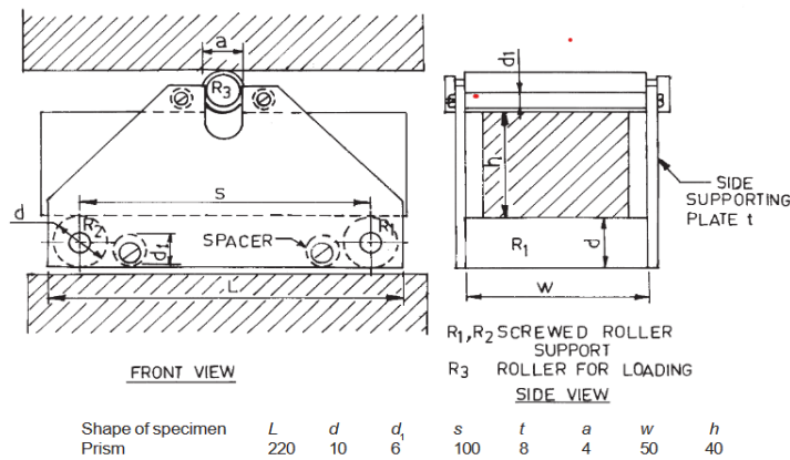
Figure 1-Steel Jig for Modulus of Rupture Test.
